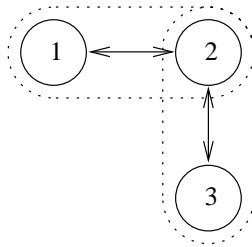
Figure 2: Example showing that Assertion 4 sometimes requires disconnected (or partially-connected) nodes to be in the same group.
