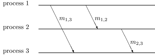
Figure 1: Example of causally-ordered delivery
