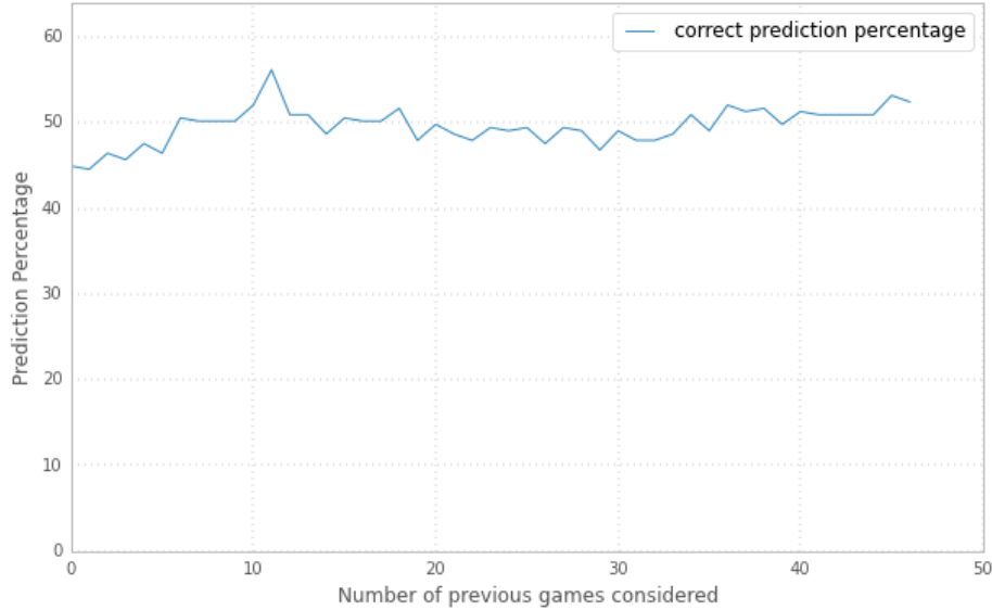
Fig. 4: Variation of accuracy with number of previous game considered for prediction.
