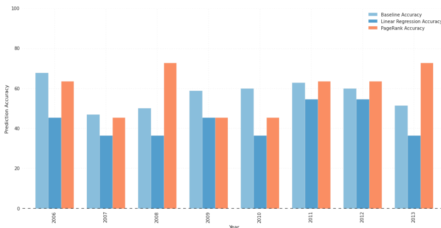
Fig. 15: Comparison of accuracy of three models used for college football.
