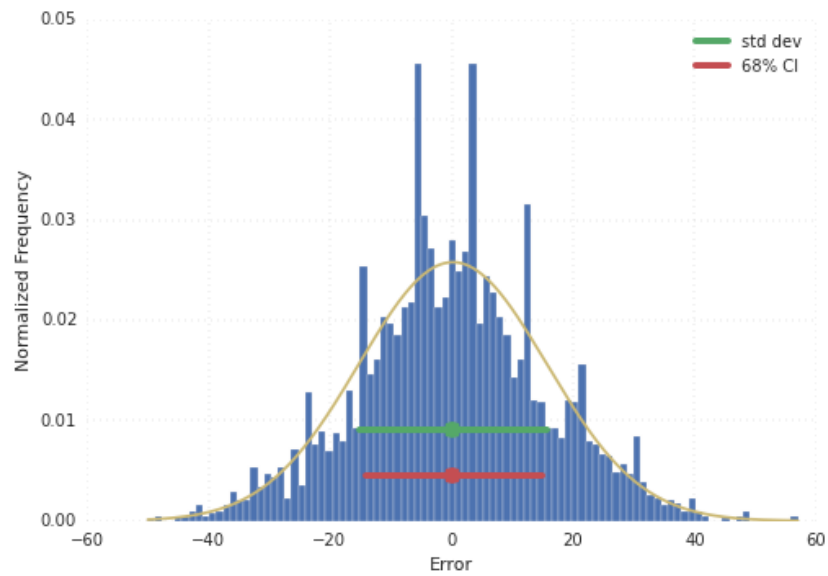
Fig. 6: Error distribution of the predicted point difference for NFL.
