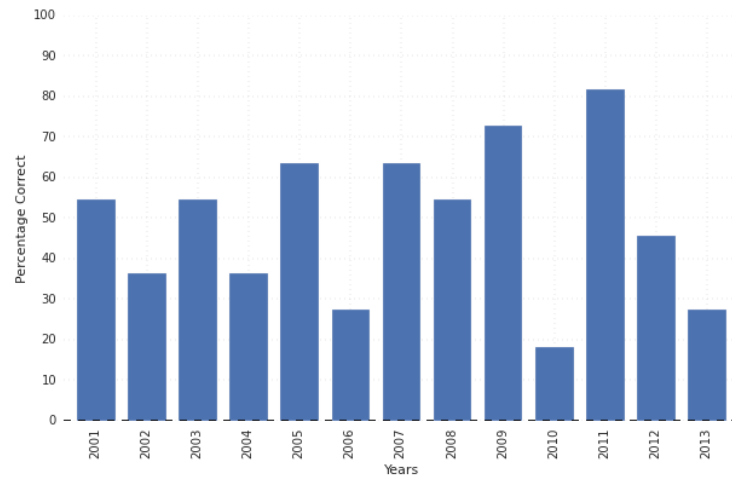
Fig. 7: Accuracy for NFL linear regression model for 14 years of data.
