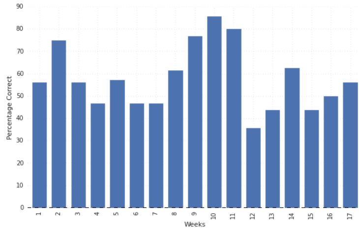
Fig. 9: Weekly accuracy for NFL linear regression model for 2014 regular season games.
