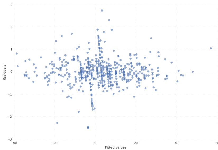
Fig. 5: Residual plot for linear regression on NFL. Residuals are spread randomly, which suggests the model fits the data well. Here the intensity of the colour represents the density of values.
