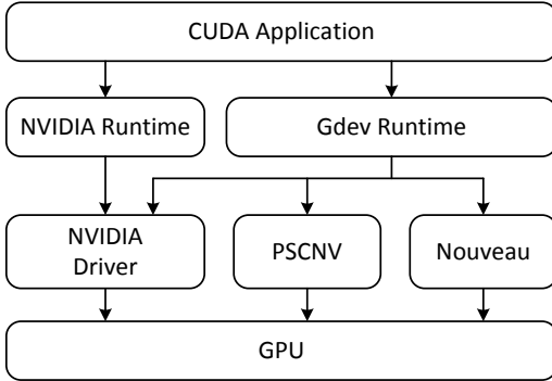
Figure 2: Structure of CUDA applications on top of the NVIDIA (closed-source) and Gdev (open-source) sets of GPGPU runtime and driver software.
