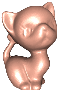
Topological Torus
