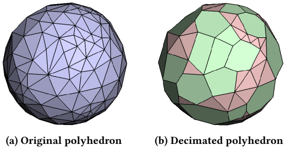
Figure 4: One round of decimation conducted on a polyhedron. Green colored faces with a vertex are removed.
