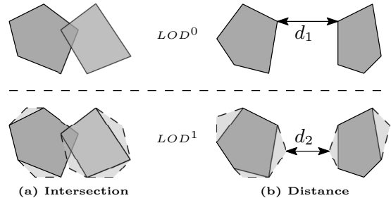
Figure 6: Properties of querying multiple LODs
