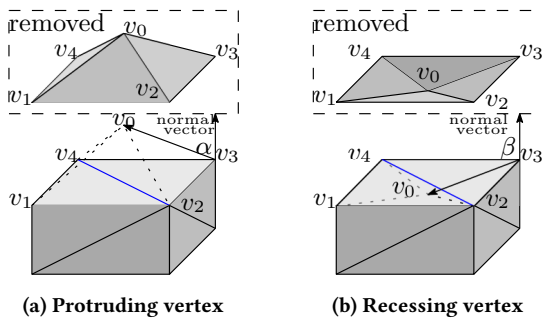
Figure 5: Protruding and recessing vertices
