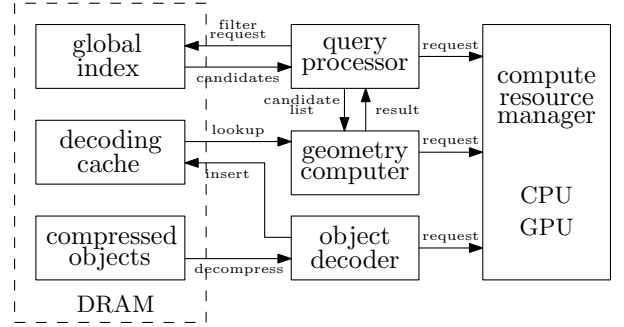
Figure 8: Overview of the architecture of 3DPro
