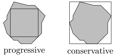
Figure 2: Two types of spatial object approximations
