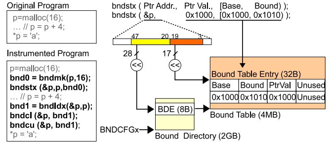
Figure 1. MPX stores the base and bound metadata ( 0x1000-0x1010 ) of the pointer p (with an initial value of 0x1000 ) in the two-level Bound Tables, and checks if the later use of pointer p (with a new value, say 0x1004 , after some updates) is within the base and the bound.
