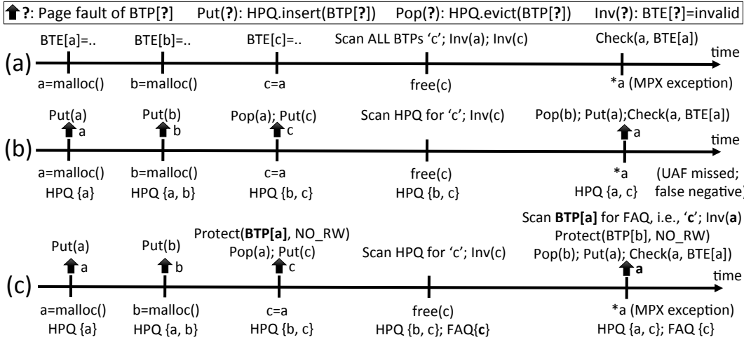
Figure 2. (a) FullScan; (b) PartialScan only; and (c) PartialScan and PageFaultScan. (b) misses the use-after-free error, and (c) solves the problem with PageFaultScan. For brevity, (b) and (c) omit the bound creation and propagation. A bold up-arrow represents a BTP fault. Put and Pop insert/evicts a BTP to/from HPQ. Inv invalidates a BTE.
