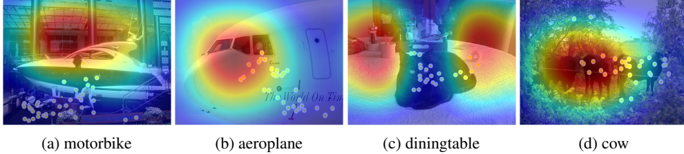
Figure 3: Failure cases. Representative images where the priority maps produced by SDR are significantly different from human fixations. The caption under each image indicates the target category. The modes of failure are: (a) failure in classification; (b) and (c) existence of a more attractive object (text or face); (d) co-occurrence of multiple objects. Best viewed on digital devices.
