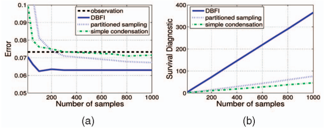
Fig. 4. Tracking results obtained for the conventional Condensation, partitioned sampling and the proposed DBFI method. Analysis of the three algorithms when applied to the tracking example explained in Section 4, which was a 20-iteration sequence. The analysis is done (a) in terms of the error in the tracking (distance between the true state and the state estimated by the algorithm) and (b) in terms of the survival rate. In both cases, the experiments have been realized for different numbers of samples and, for each specific number of samples, 25 repetitions of the simulation have been performed. The results we show correspond to the mean of these 25 repetitions, with 20 iterations each. Observe that the results agree with the a posteriori distributions plotted in Fig. 2 as DBFI outperforms both the Condensation and the partitioned sampling algorithms.
