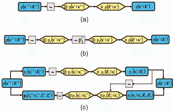
Fig. 3. Whole process diagrams of the conventional Condensation, the partitioned sampling, and the DBFI algorithms. The symbology used in these diagrams is adapted from [17]: \sim denotes the resampling operation, \sim p_i^i indicates a weighted resampling operation with respect to the importance function p_i^i , \otimes represents a convolution operation with the dynamics, and \times is the multiplication by the observation density (see [17] for details). (a) Conventional condensation x = [x_1, x_2] . (b) Partitioned sampling x = [x_1, x_2] . (c) DBFI.
