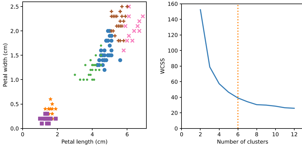
(a) 2D representation of the Iris dataset, plotting only petal width vs. petal length. Six clusters were chosen using the elbow method. Each color and marker represents a different cluster.
