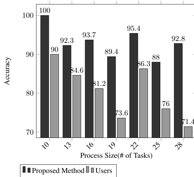
Fig. 7: Relation Between Accuracy and Process Size
