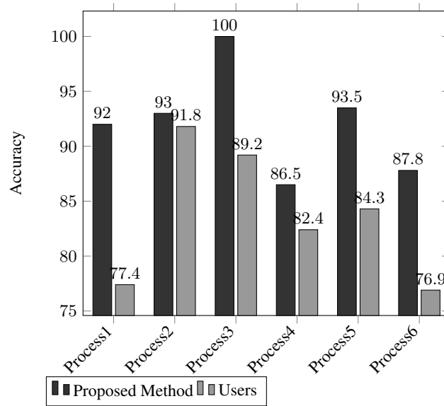
Fig. 6: Accuracy Comparison using several processes
