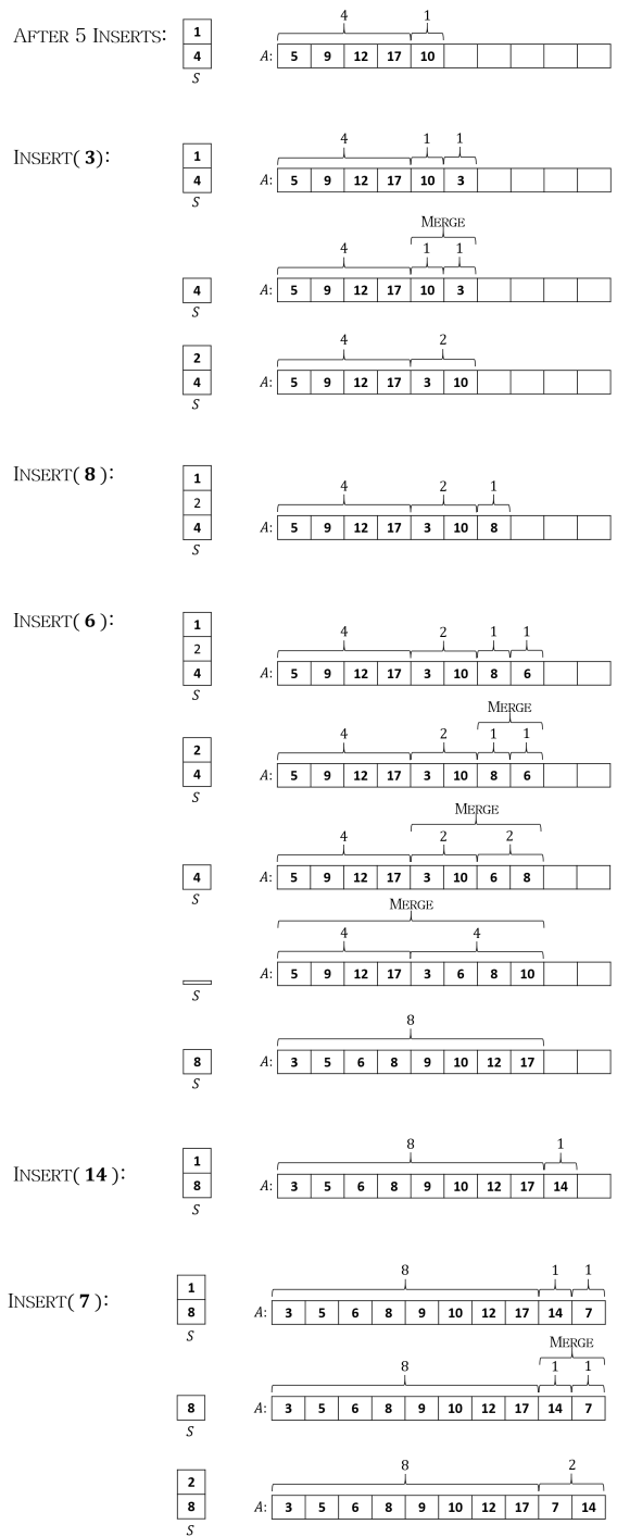
Figure 3: An example showing how the data structure works (ref: question 3).
