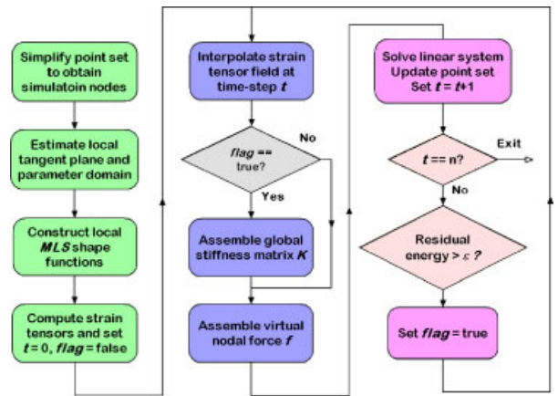
Figure 5. Algorithmic overview and flowchart.
