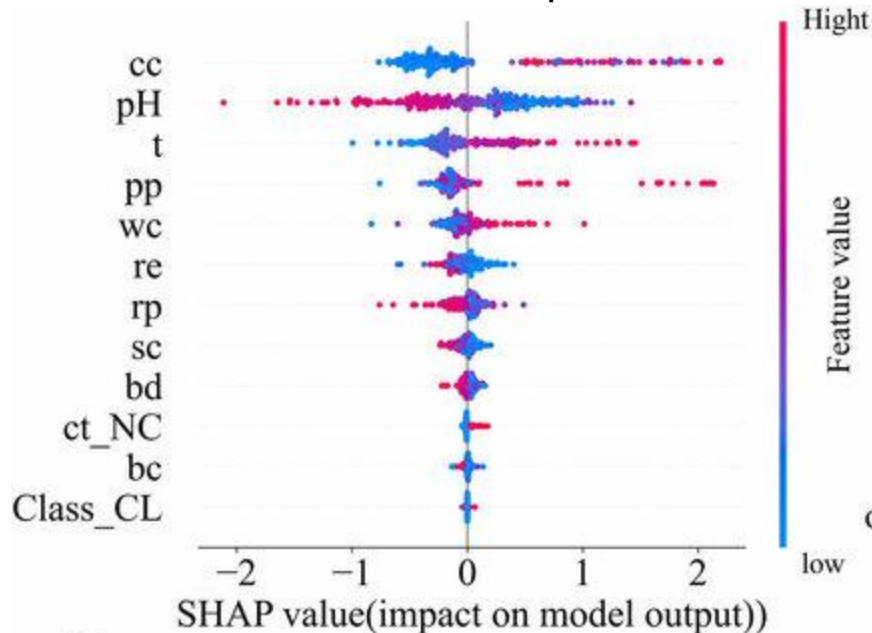
SHAP Beeswarm plot
