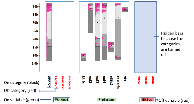
Figure 5: The Parameter Explorer in action for the system performance dataset. Analysts can select parameters from the Parameter Explorer and visualize throughput distributions and statistics in real time.
