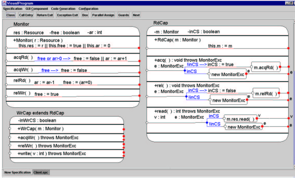
Figure 1. Package ReaderWriter.
