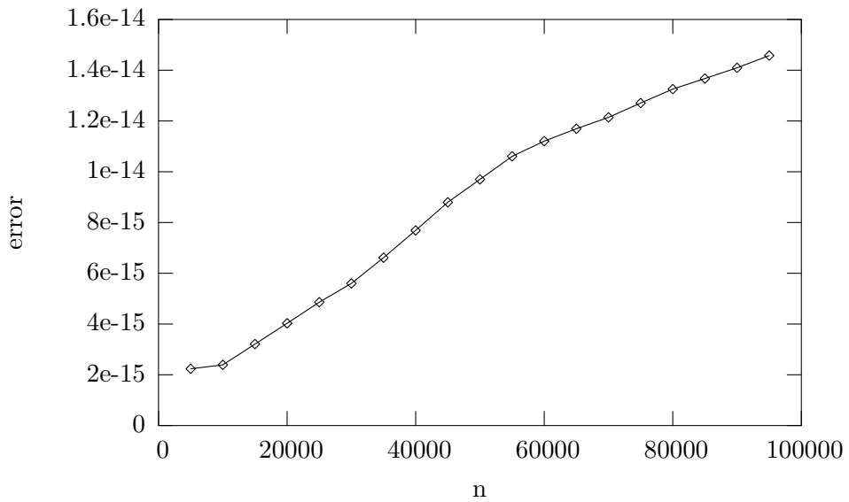
Figure 13: Relative error for sequence local average with k=1000.
