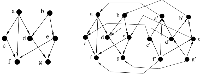
FIG. 5 The original DAG G is on the left. On the right we show L constructed from G .
