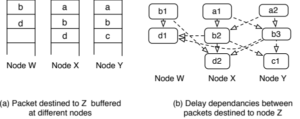
Fig. 2. Delay dependencies between packets destined to Z buffered in different nodes.
