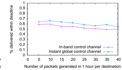
Fig. 14. (Trace) Global channel: Packets delivered within deadline increases by about 15% using instant global control channel
