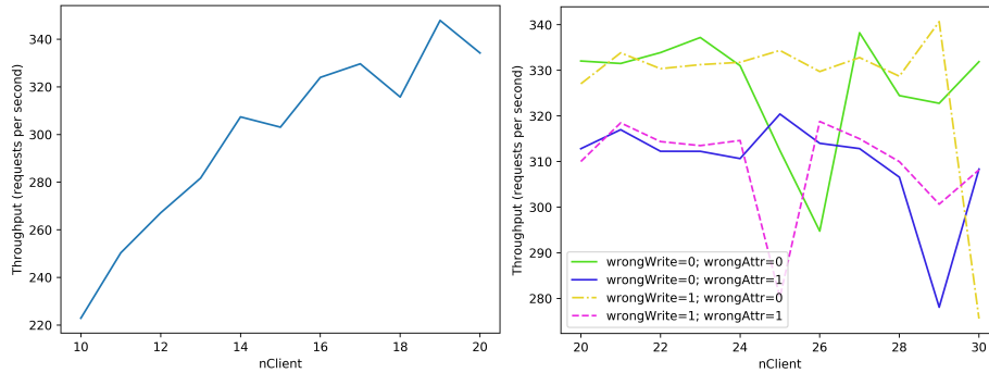
Fig. 6. Average throughput as a function of nClient for Decat et al. 's algorithm (left) and FACADE (right).
