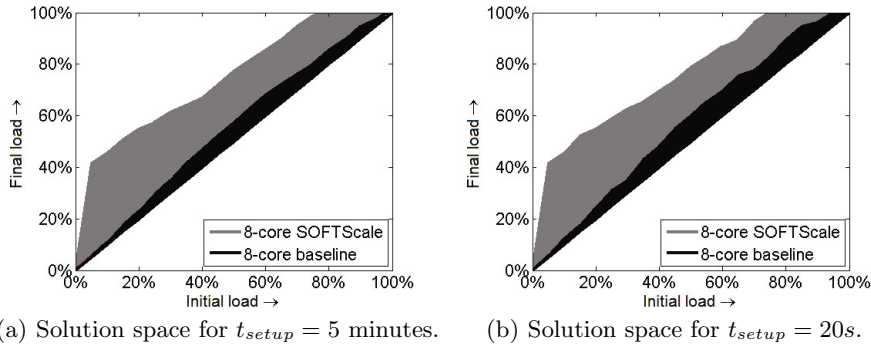
Fig. 16. Full range of results for SOFTScale with 8-core memcached servers under (a) t_{setup} = 5 minutes and (b) t_{setup} = 20s . We see that 8-core memcached servers provide huge benefits for SOFTScale regardless of the setup time.
