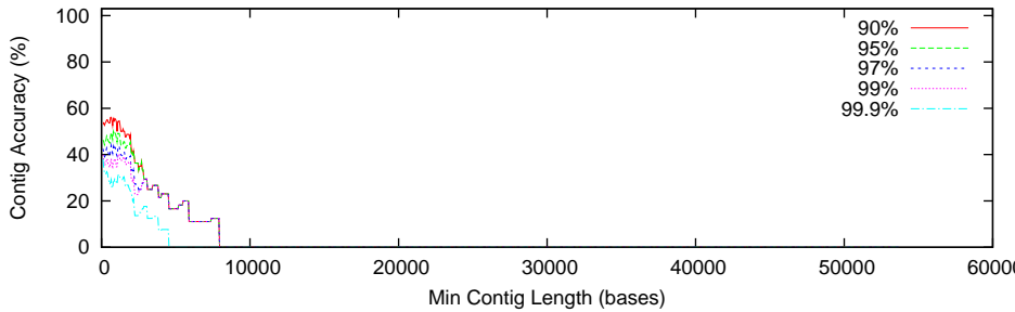
Min Contig Len-Contig Accuracy Plot
