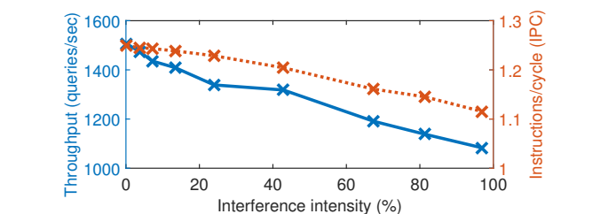
Fig. 1: Empirical results for decrease in throughput and IPC as a function of interference intensity.
