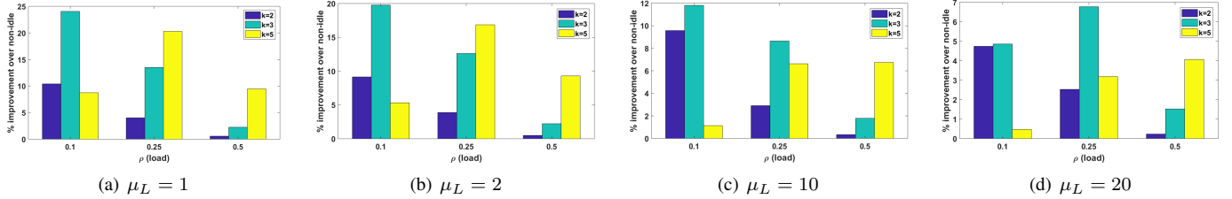
Fig. 10: Improvement over non-idling policy for 2, 3, and 5-VM systems; \mu_H = 100 , \alpha_L = 1/10 , \alpha_H = 1 , \mu_L \in \{1, 2, 10, 20\} .
