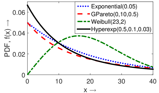
Fig. 1: Illustration of the probability distribution function (PDF) of various distributions, all with mean 20.
