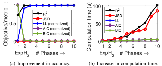
Fig. 10: Impact of number of phases on (a) improvement in accuracy, and (b) computation time, for different techniques/objectives. Note that phase = 1 refers to Exponential and phase = 2 refers to 2-phase Hyper-exponential ( H_2 ).
